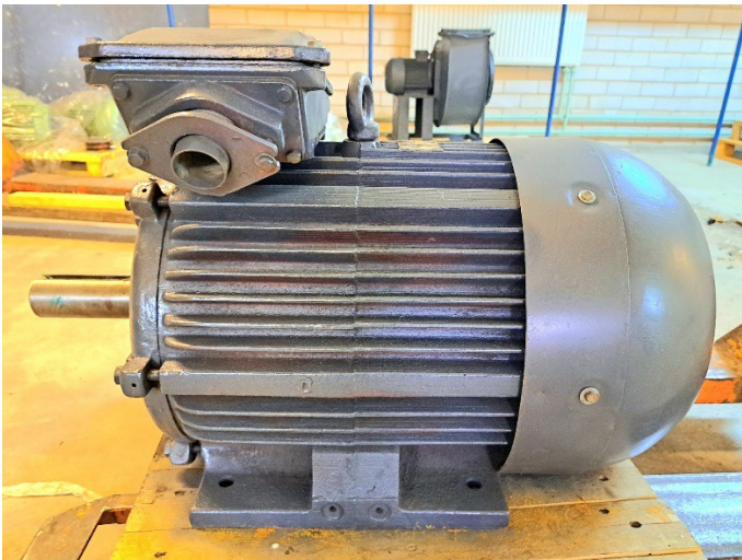
4A200B6 30kW, 960 aps/min, 220/380V Kaina 650,- EUR be PVM.
