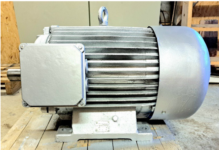
IMB3-200L6 22kW 925 aps/min 220/380V Kaina 700,- EUR be PVM.
