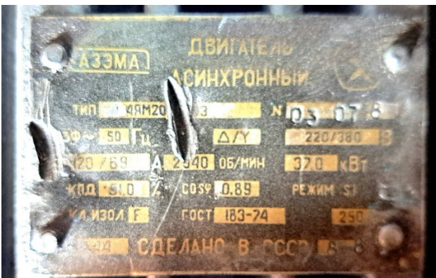
4AM200B2, 37kW, 2940aps/min, 220/380V
