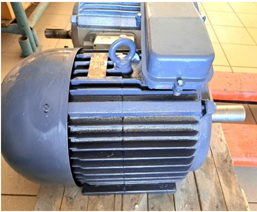
18,5kW, 975aps/min, 220/380V Kaina 600,- EUR be PVM.
